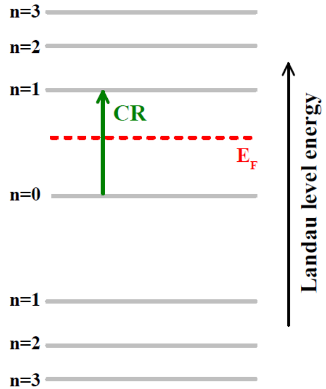
2D Dirac electrons
